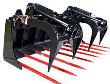
BALE FORK GRAPPLE (BFG885)
